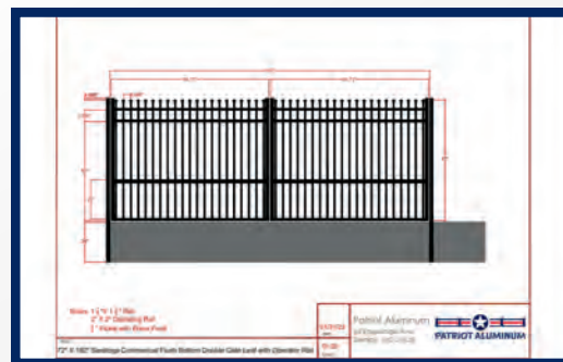
Double Swing Gate Drawing
