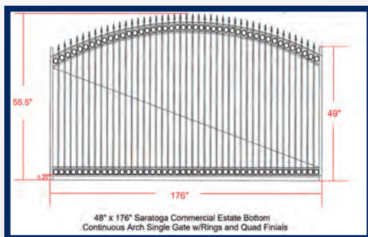
Single Estate Gate Drawing
